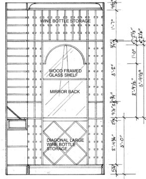
C WINE ROOM: ELEVATION SCALE: 1/4" = 1'-0"
