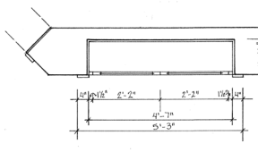
B DINING ROOM: BUILT-IN CHINA CABINET PLAN SCALE: 1/4" = 1'-0"
