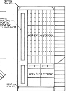
B WINE ROOM: ELEVATION SCALE: 1/4" = 1'-0"
