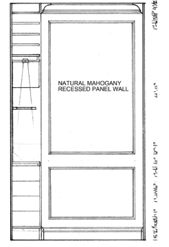
D WINE ROOM: ELEVATION SCALE: 1/4" = 1'-0"
