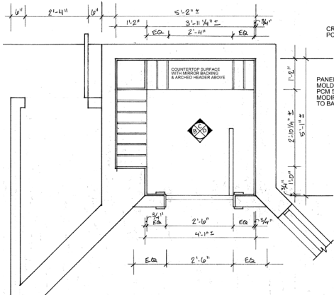
A WINE ROOM: FLOOR PLAN SCALE: 1/4" = 1'-0"
